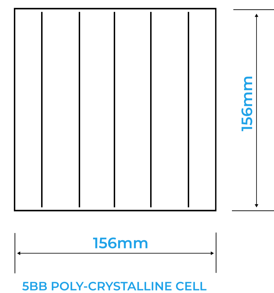
SBB POLY-CRYSTALLINE CELL
